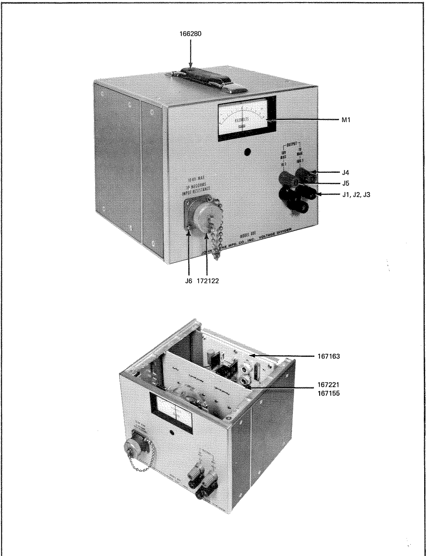
Figure 5-1. FINAL ASSEMBLY
